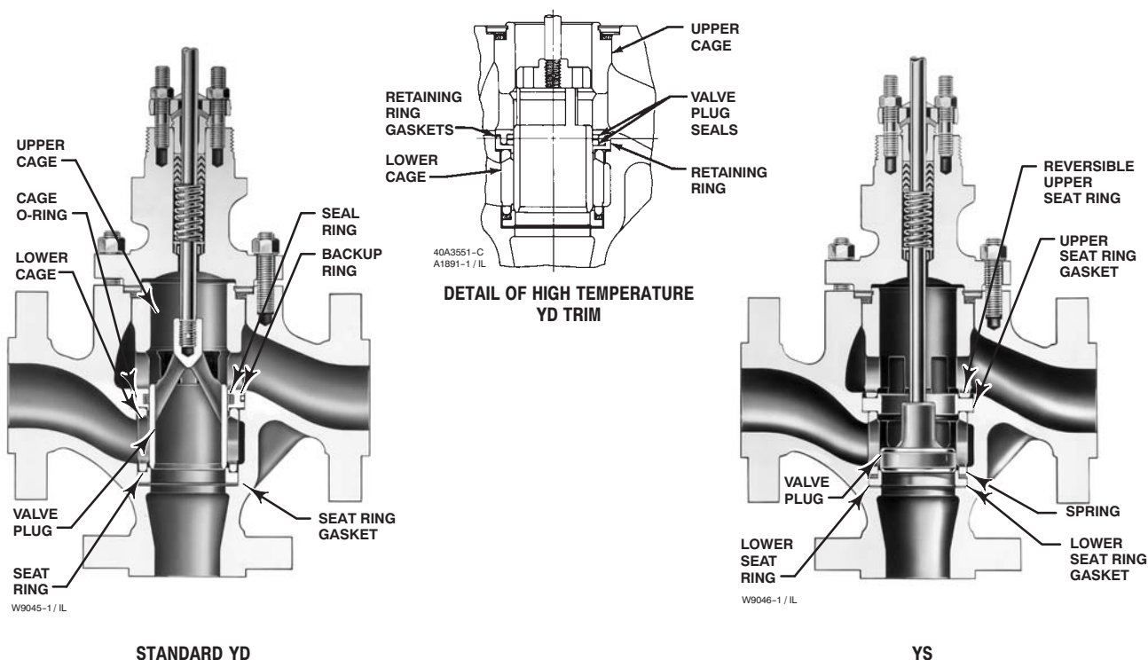
Figure 2. Construction Details
