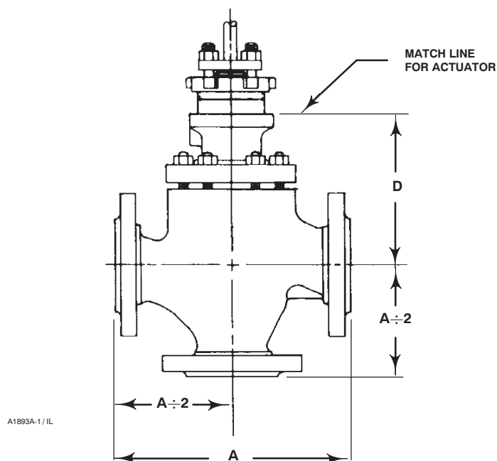
Figure 7. Fisher® YD and YS Dimensions (also see table 9)
