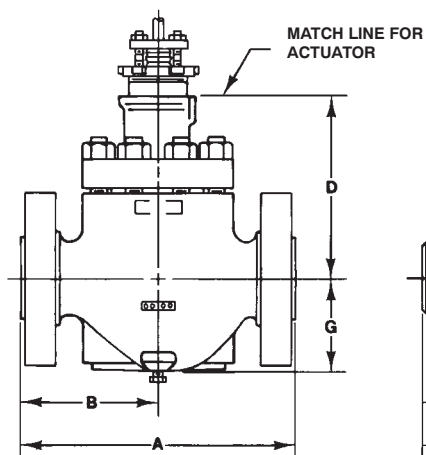
FLANGED VALVE WITH 71 OR 90 mm (2-13/16 OR 3-9/16 INCH) DIAMETER YOKE BOSS
