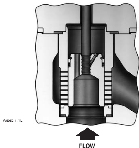
Figure 10. Fisher® HPT Trim with Whisper Trim® III Level A1 Cage (Available in HPD [NPS 2-6] and HPS [NPS 2 and 3])
