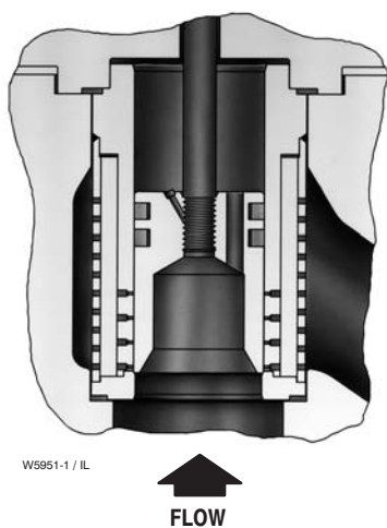
Figure 11. Fisher® HPD Trim with Whisper Trim® III Level D Cage
