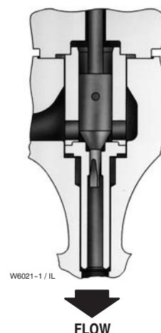
Figure 12. Fisher® HPAS Trim with Micro-Flat Valve Plug
