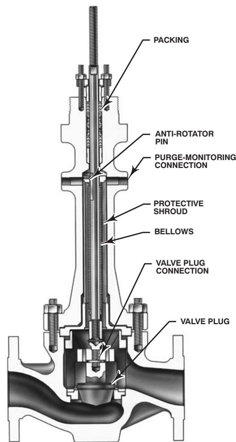
Figure 3. Fisher® EZ Valve with ENVIRO-SEAL® Bellows Seal Bonnet
