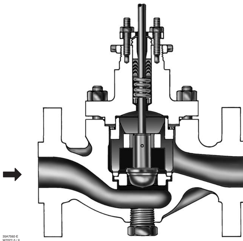
Figure 2. Fisher® EZ Sectional
