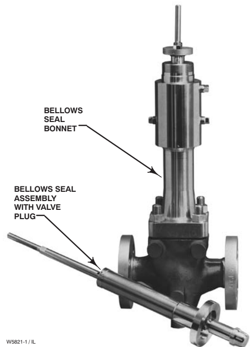
Figure 10. Typical ENVIRO-SEAL® Bellows Seal Bonnet and Bellows Seal Assembly
