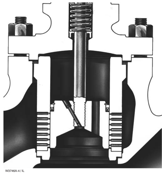
Figure 9. Cavitrol® III One-Stage Cage
