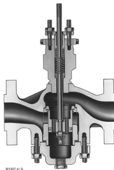
Figure 4. Fisher® ETR Sectional
