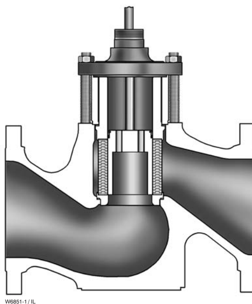
Figure 4. Fisher® ETR Sectional
