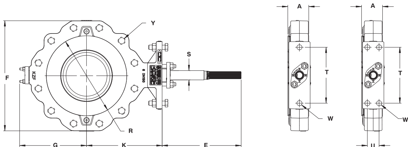
Figure 8. Dimensions for Fisher® 8580, Single Flange Valve
