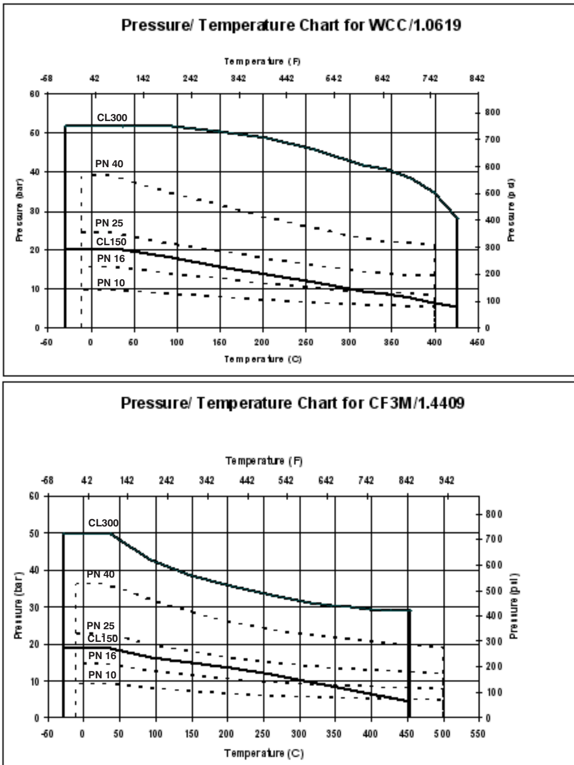
Figure 6. Material Pressure/Temperature Curves
