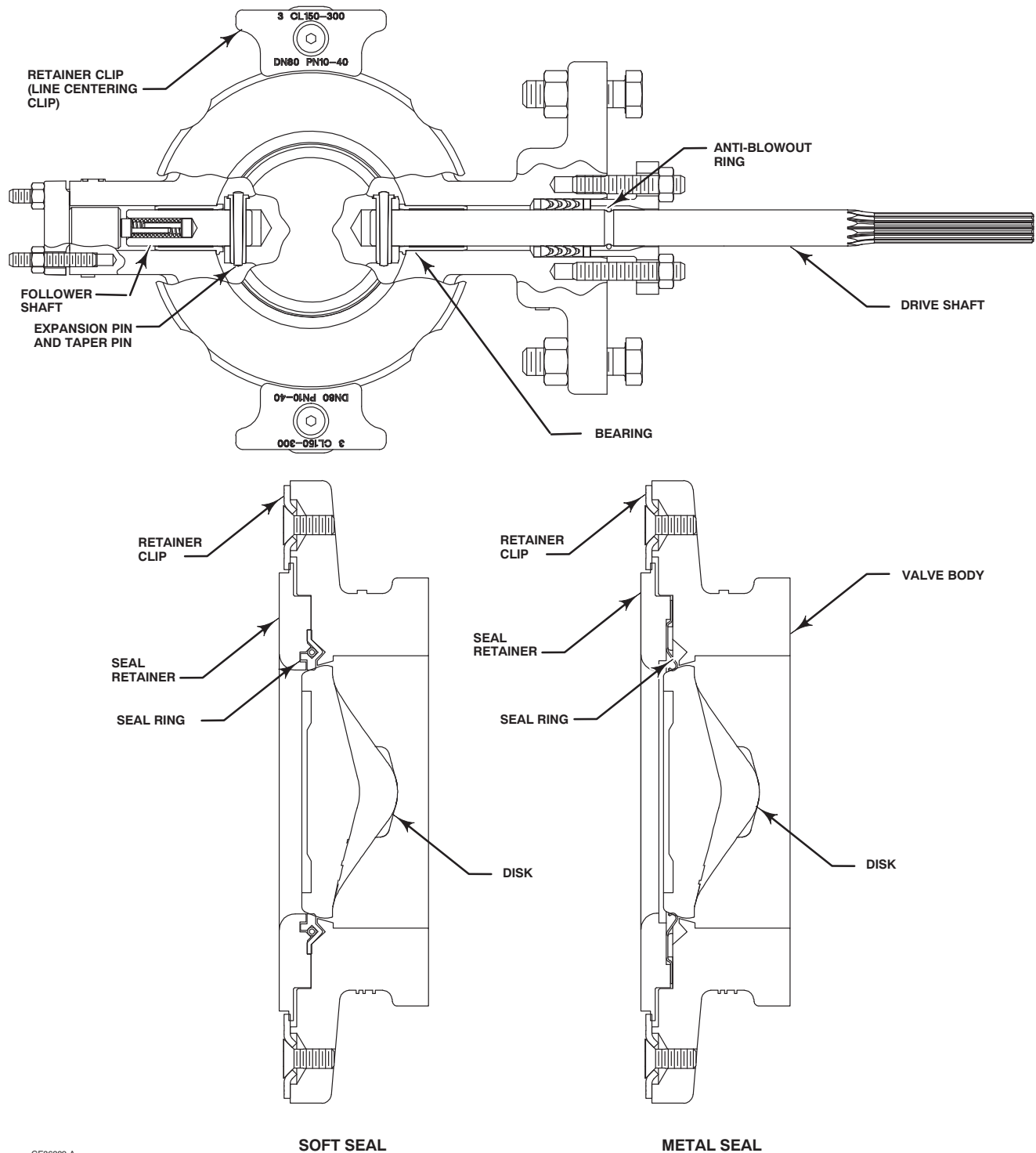
Figure 2. Typical Fisher® 8580 Valve Construction Detail
