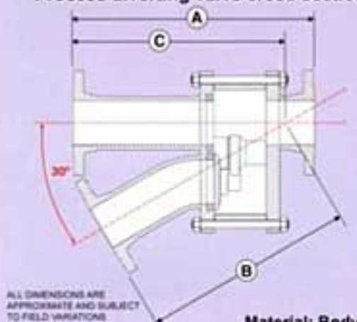
Process diverting valve cross section
