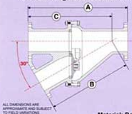
Cast diverting valve cross section
