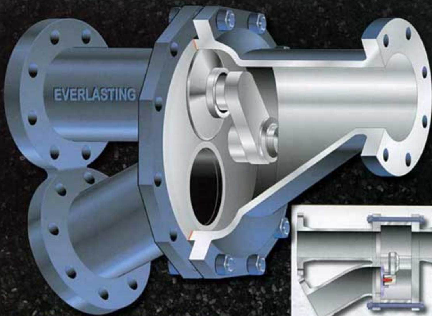
PROCESS DIVERTER
